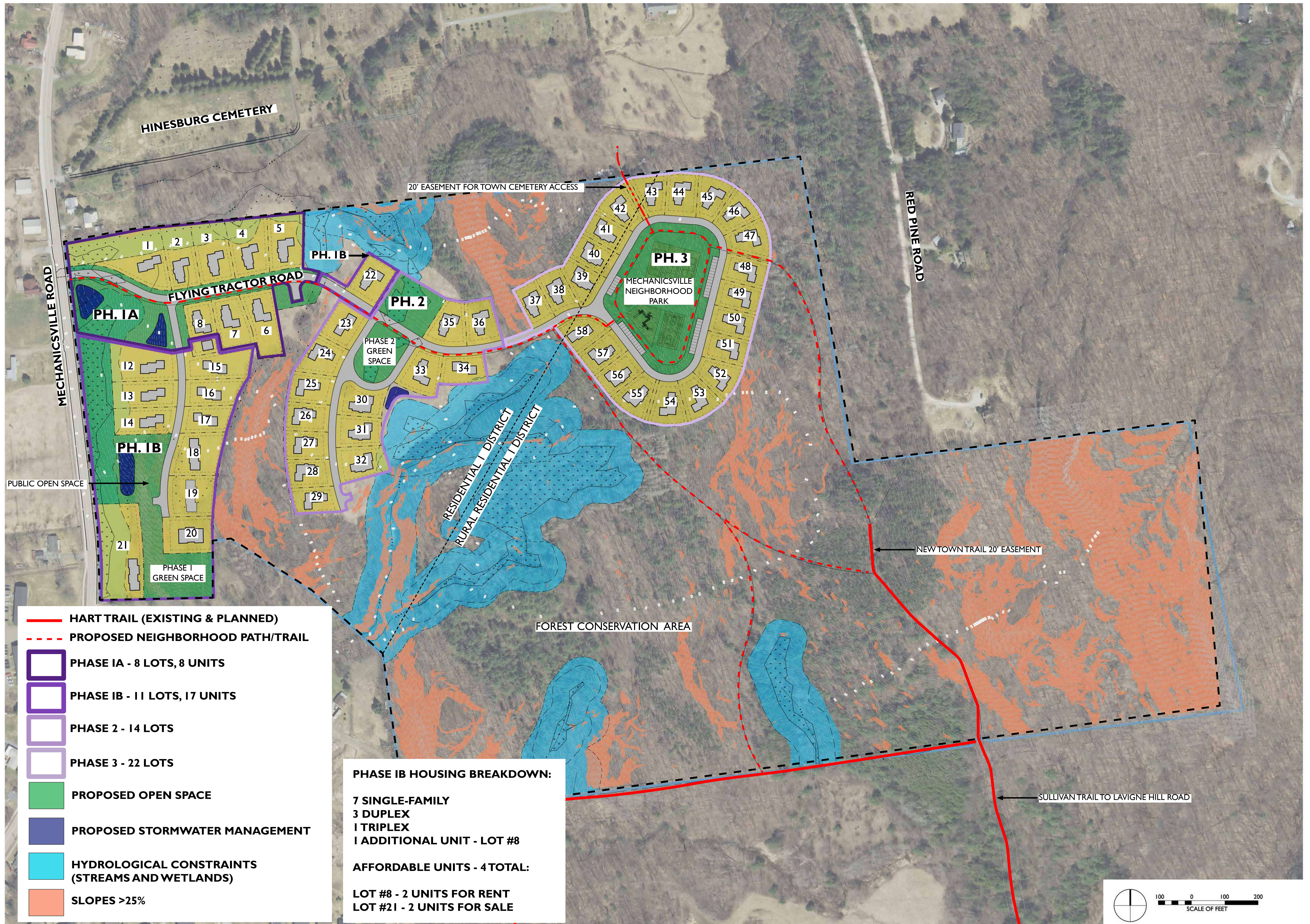
LASTER SUBDIVISION | PROPOSED LOT LAYOUT WITH PHASING
